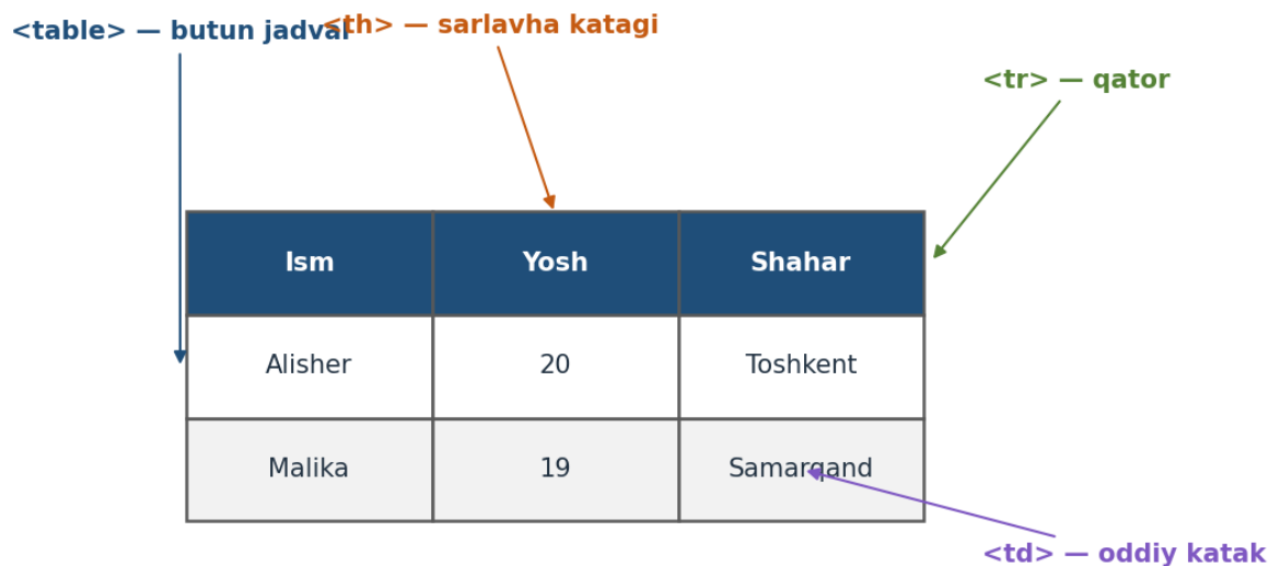
11-rasm. HTML jadval teglari
